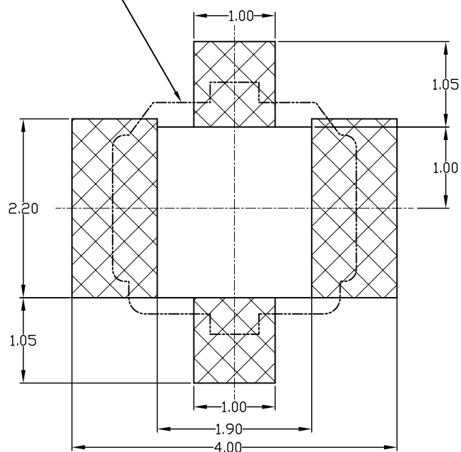
RECOMMENDED FOOTPRINT PATTERN
