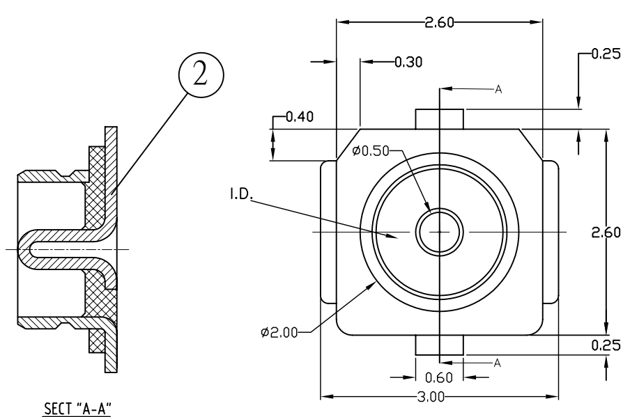
CONNECTOR OUTLINE
