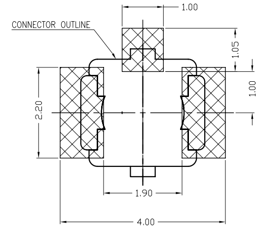
RECOMMENDED FOOTPRINT PATTERN
