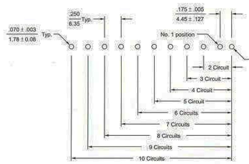
P.C. board hole dimensions
