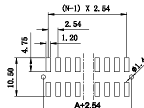
P C B Layout
