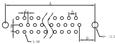
26,44,62 POSITION MALE
