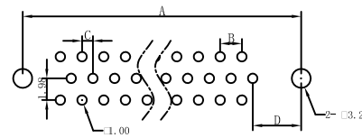
26,44,62 POSITION FEMALE
