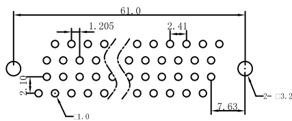
78 POSITION FEMALE/MALE
