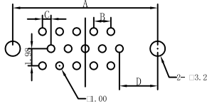
15 POSITION FEMALE
