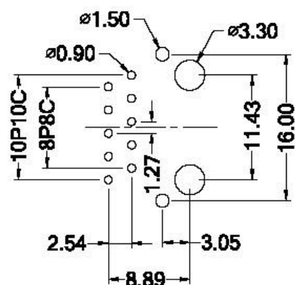
PCB LAYOUT / TOP VIEW / R3.05
