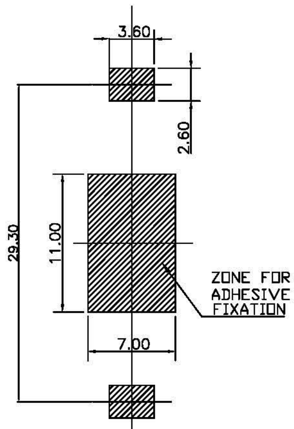
PCB LAYOUT
