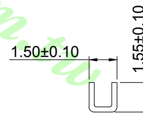
C-C SECTION
