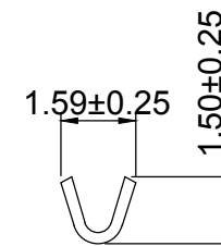
B-B SECTION
