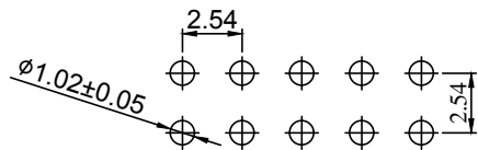
Recommended P.C.Board Hold Layout
