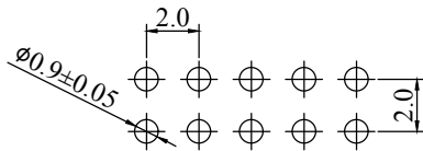
Recommended P.C.Board Hold Layout
