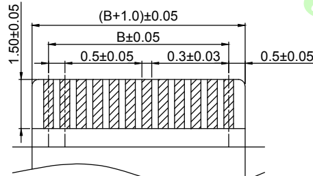
APPLICABLE FFC DIMENSION(REF) THICKNESS 0.30 +0.02 / -0.00
