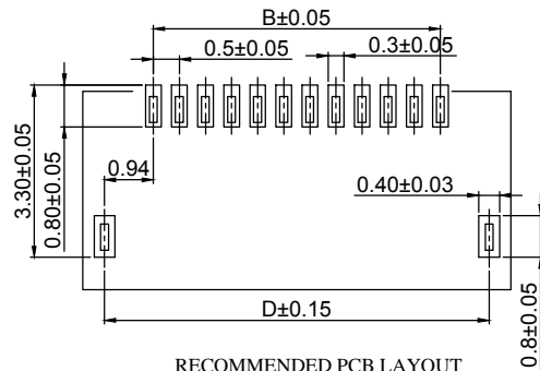
RECOMMENDED PCB LAYOUT TOLERANCE±0.05 (N=CIRCUITS)
