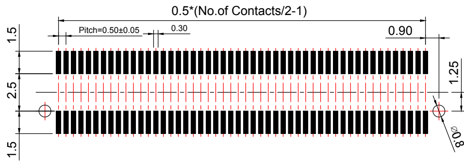
PCB Layout For Surface Mounting
