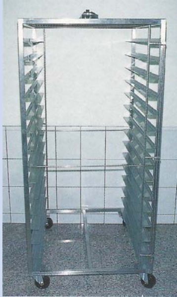
烤爐用檯車附自動懸吊裝置 Trolley for rack oven with lifting device.
