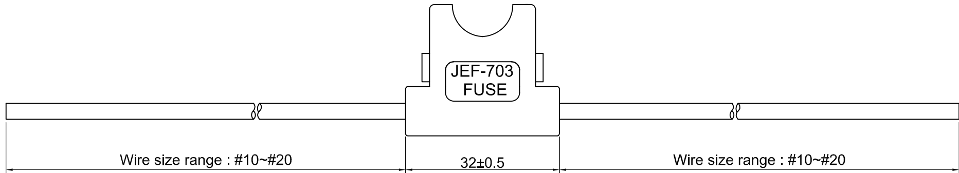
FUSE HOLDER BLACK COLOR
