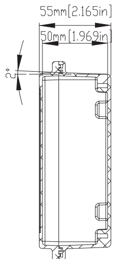
SECTION C-C
