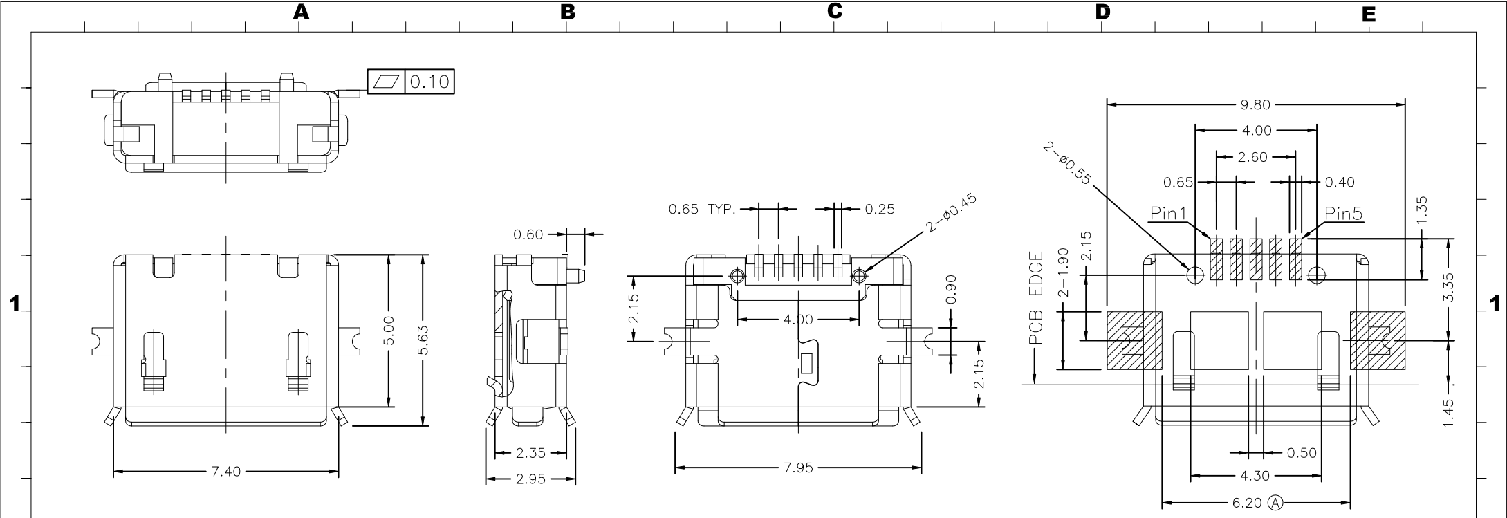
P.C.B LAYOUT TOP VIEW ±0.05
