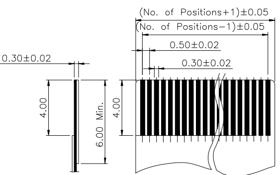
FFC/FPC Dimension(Thickness 0.30 mm)
