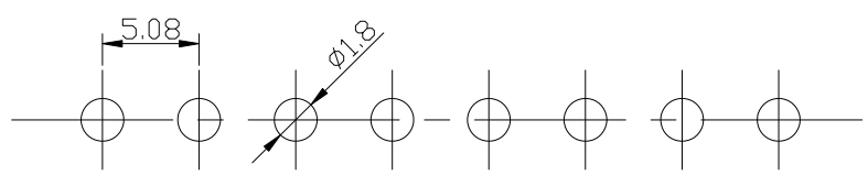
RECOMMENDED P.C.BOARD HOLE DIM.
